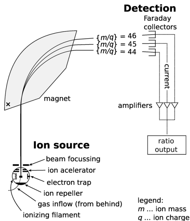
Figure 33. Schematic picture of mass spectrometer. (Adapted from: Mesuere et al., 2016 50 )
